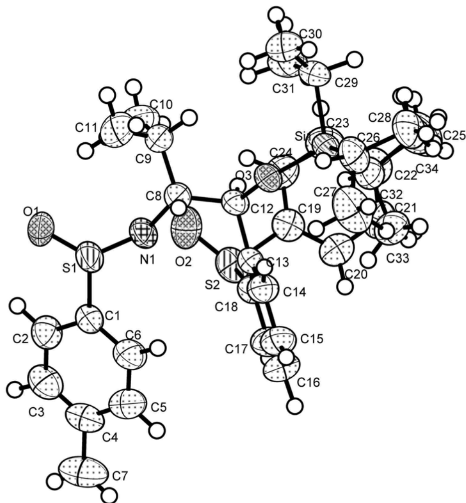
Figure 1. Ortep diagram for compound of 3i
